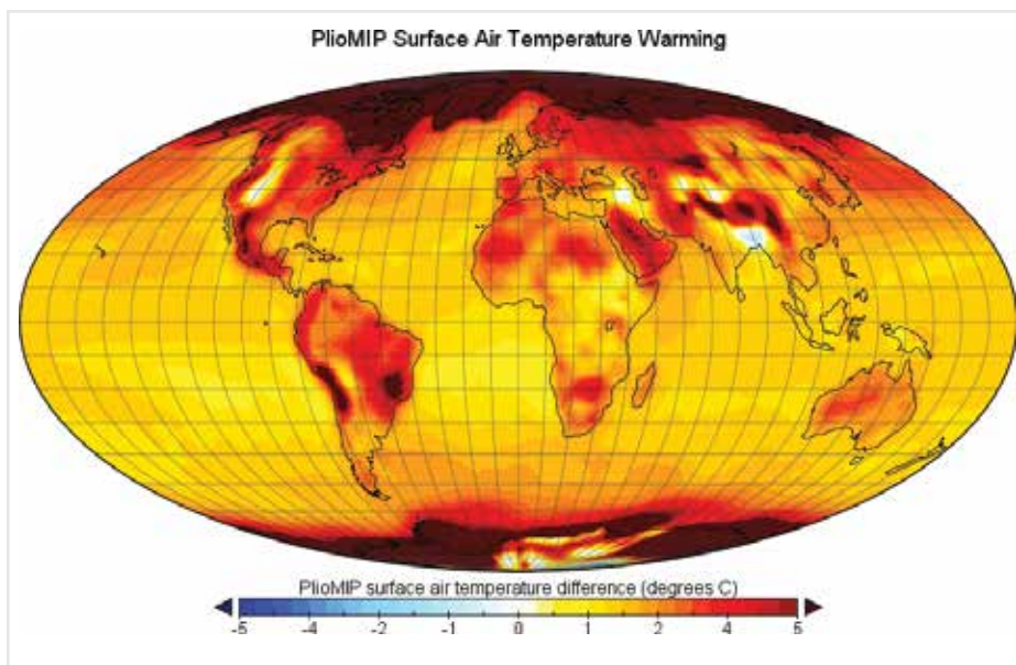
Figure 1: Mean annual surface air temperature anomaly (mid-Pliocene minus pre-industrial simulations) based on a multi-model means ensemble obtained by the Pliocene Model Intercomparison Project. Adapted from Haywood et al. (2013).
