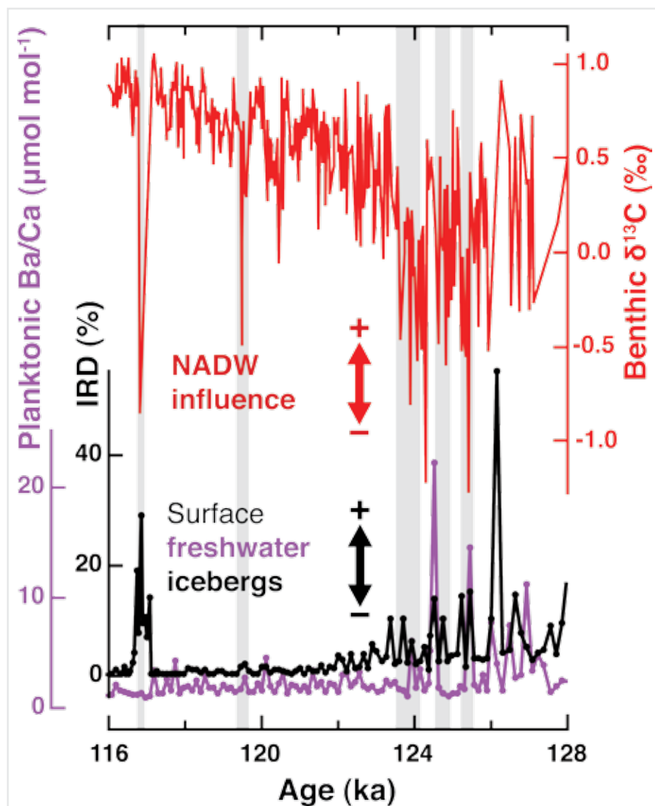
Figure 2: Eirik Drift sediment core MD03-2664 records across the LIG, focused on the Marine Isotope Stage 5e benthic \delta^{13}\text{C} plateau, (116.1-128.0 ka; Shackleton et al. 2002; Shackleton et al. 2003): Red curve: \delta^{13}\text{C} measured on shells of the epibenthic foraminifera C. wuellerstorfi ; Purple curve: Ba/Ca ratio in shells of the planktonic foraminifera N. pachyderma (s); Black curve: Ice-rafted debris (IRD) percentage in the coarse fraction. Gray shading highlights intervals of reduced bottom water \delta^{13}\text{C} and NADW influence. Figure modified from Galaasen et al. (2014).
